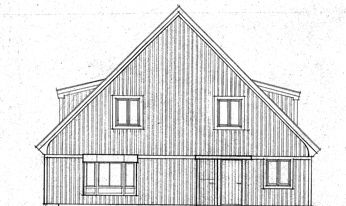
GAVELFASAD Cgvb
