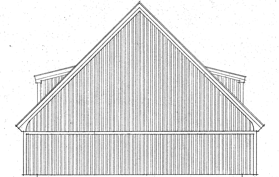
GAVELFASAD Bgv
