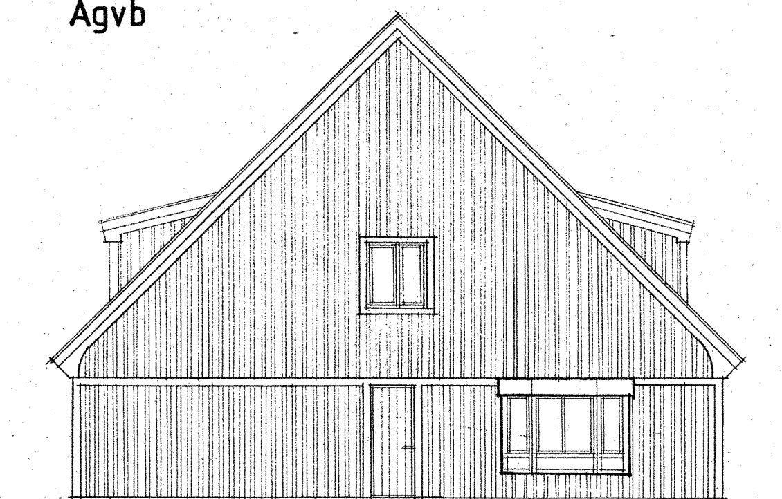
GAVELFASAD Bghb
